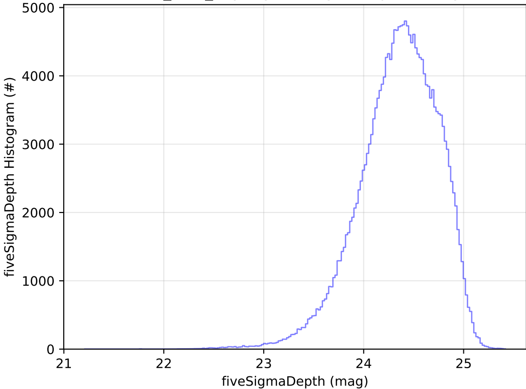
baseline_v2.1_10yrs g: fiveSigmaDepth Histogram
