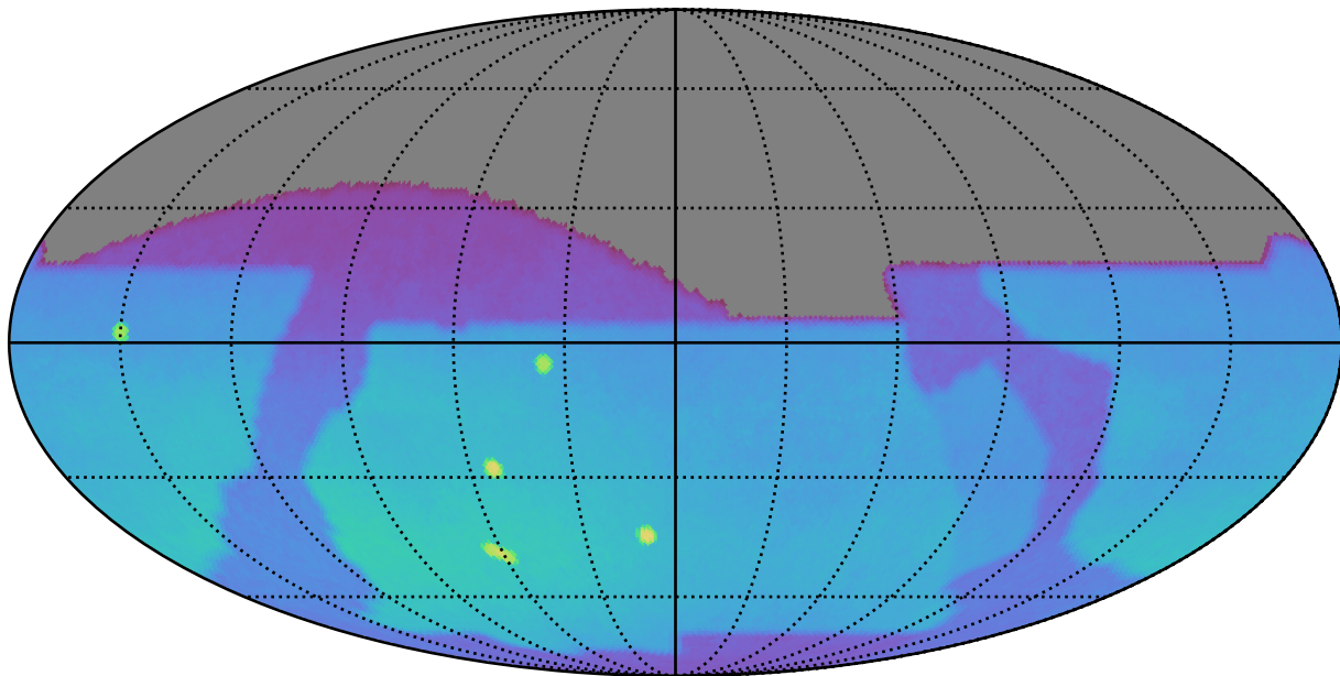
baseline_v2.2_10yrs : Brown Dwarf, L4
