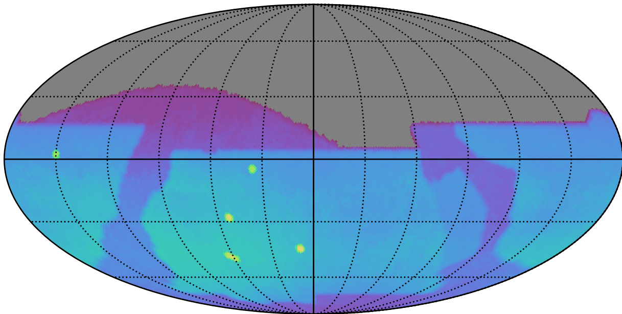
baseline_v2.2_10yrs : Brown Dwarf, L7
