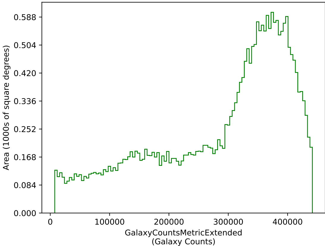
baseline_v2.2_10yrs g: GalaxyCountsMetricExtended
