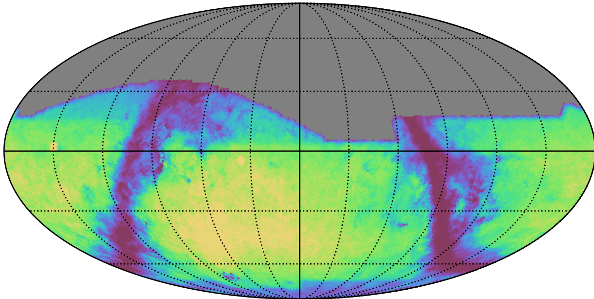
baseline_v2.2_10yrs g: GalaxyCountsMetricExtended
