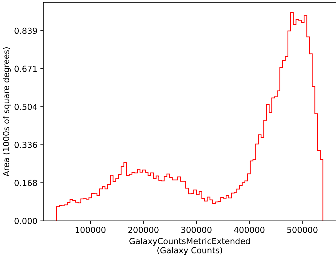
baseline_v2.2_10yrs i: GalaxyCountsMetricExtended
