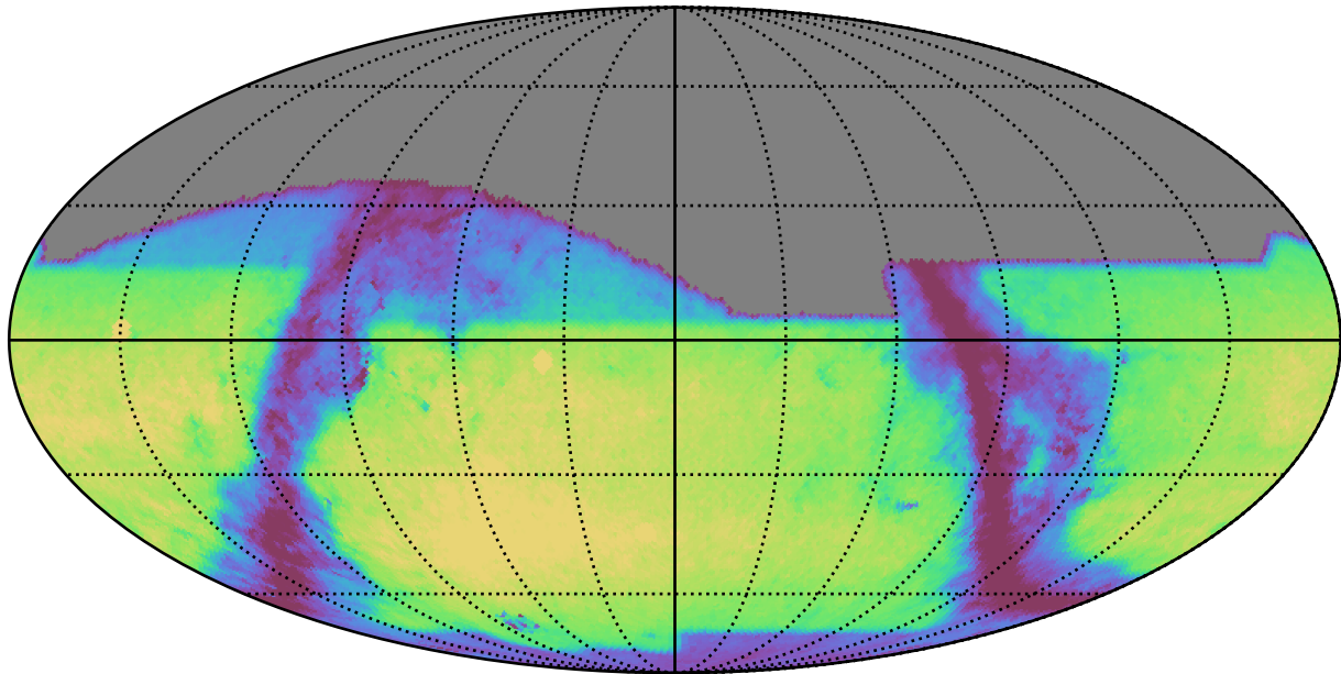
baseline_v2.2_10yrs i: GalaxyCountsMetricExtended
