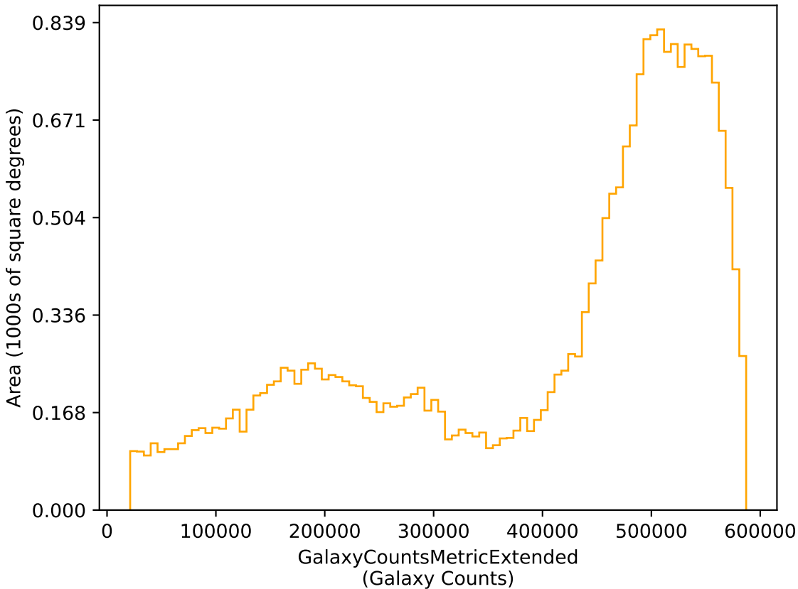
baseline_v2.2_10yrs r: GalaxyCountsMetricExtended
