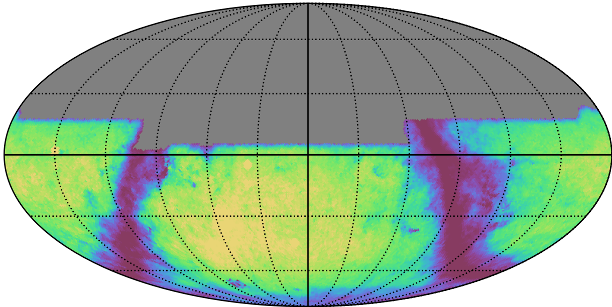
baseline_v2.2_10yrs u: GalaxyCountsMetricExtended
