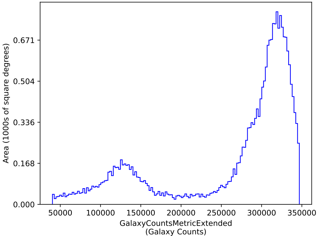
baseline_v2.2_10yrs y: GalaxyCountsMetricExtended
