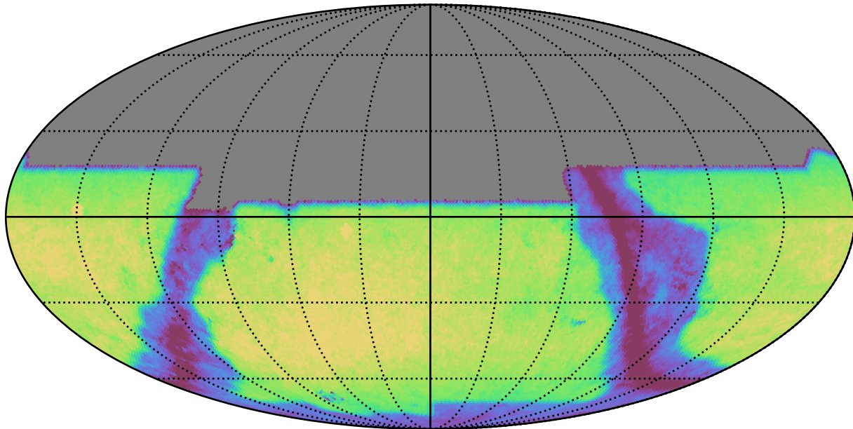
baseline_v2.2_10yrs y: GalaxyCountsMetricExtended
