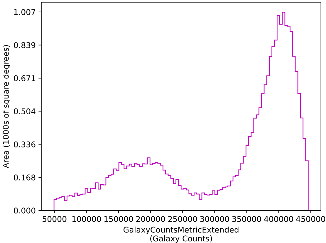
baseline_v2.2_10yrs z: GalaxyCountsMetricExtended
