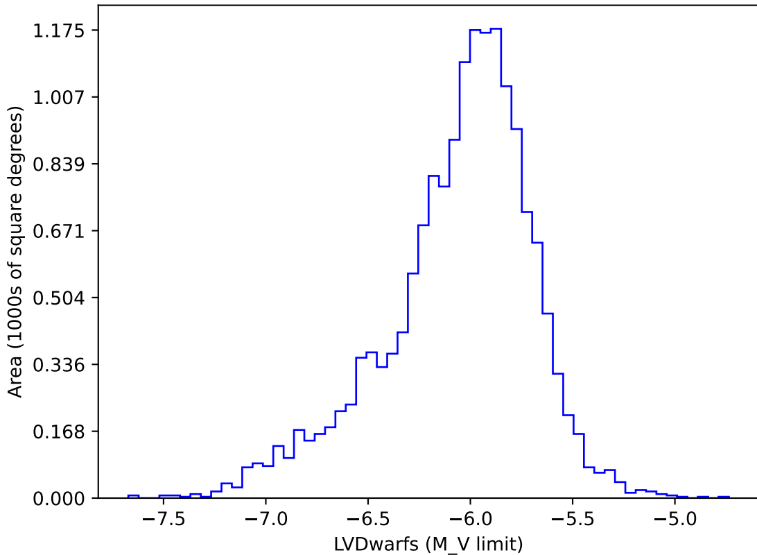
baseline_v2.2_10yrs gi: LVDwarfs
