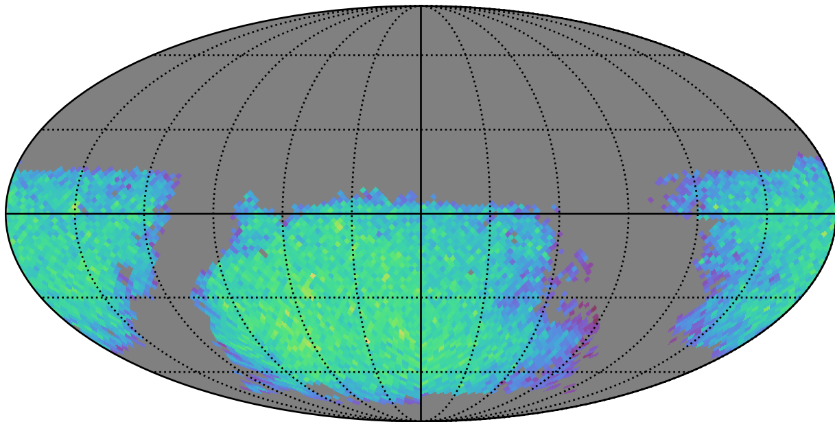
baseline_v2.2_10yrs gi: LVDwarfs
