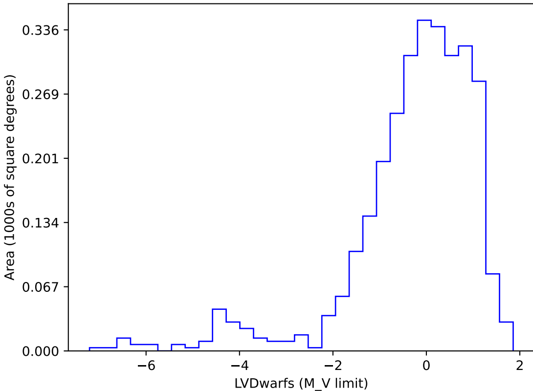
baseline_v2.2_10yrs gi SCP: LVDwarfs
