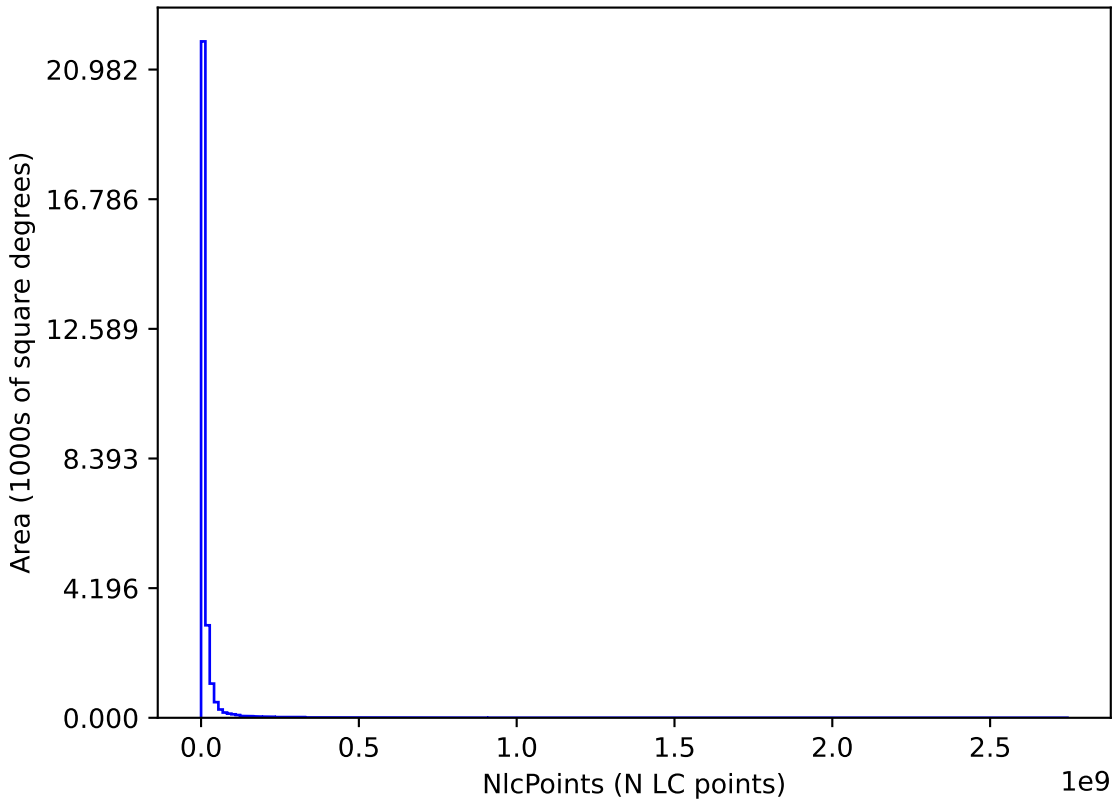
baseline_v2.2_10yrs : NlcPoints
