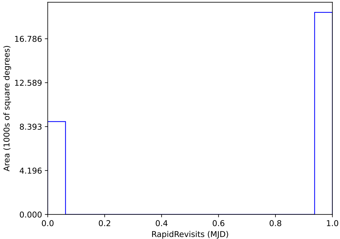
baseline_v2.2_10yrs : RapidRevisits
