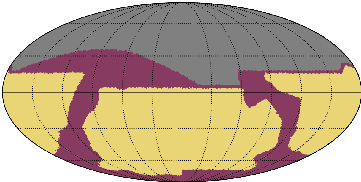
baseline_v2.2_10yrs : RapidRevisits
