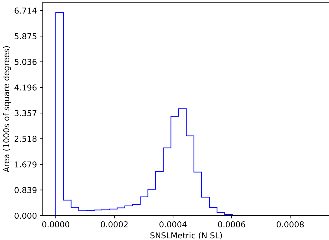
baseline_v2.2_10yrs : SNSLMetric
