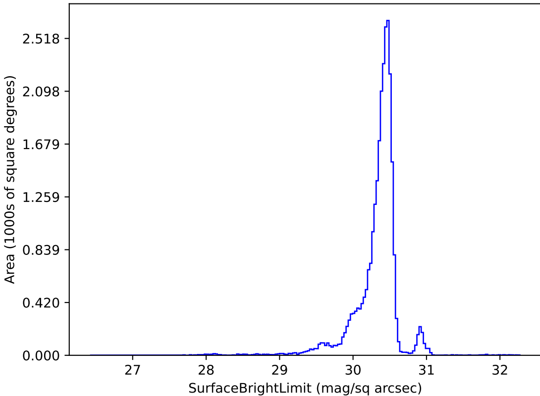
baseline_v2.2_10yrs g: SurfaceBrightLimit
