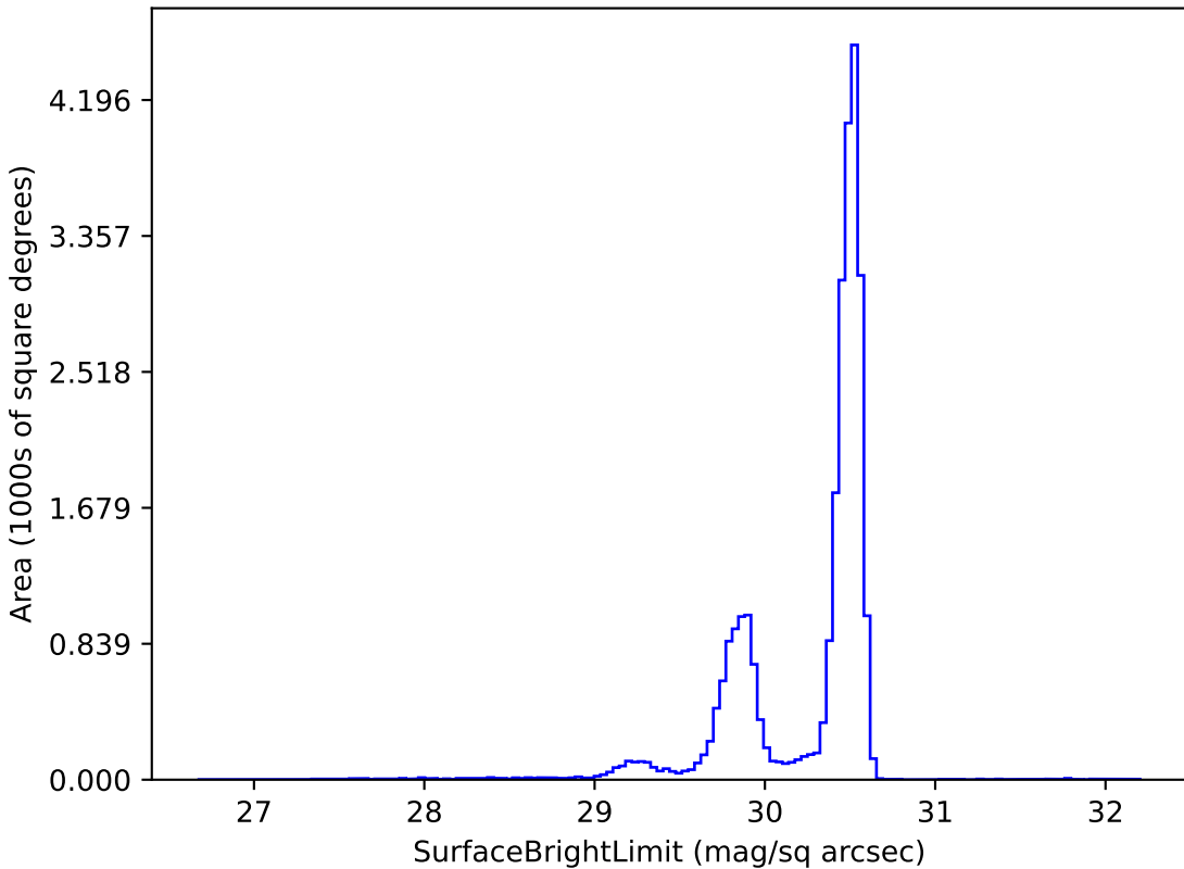
baseline_v2.2_10yrs r: SurfaceBrightLimit
