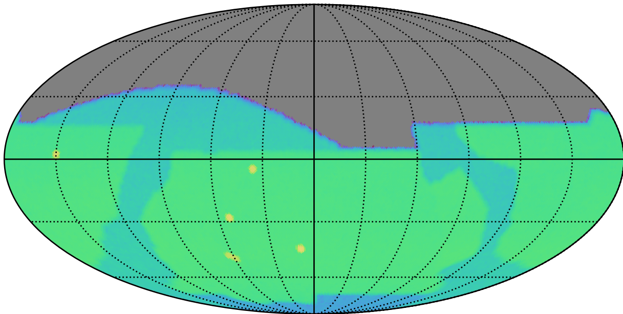
baseline_v2.2_10yrs r: SurfaceBrightLimit
