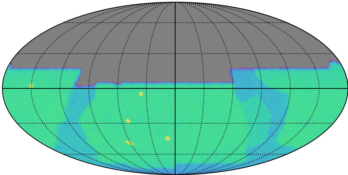
baseline_v2.2_10yrs u: SurfaceBrightLimit
