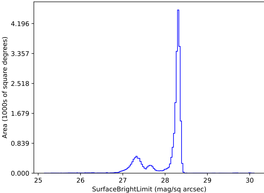
baseline_v2.2_10yrs y: SurfaceBrightLimit
