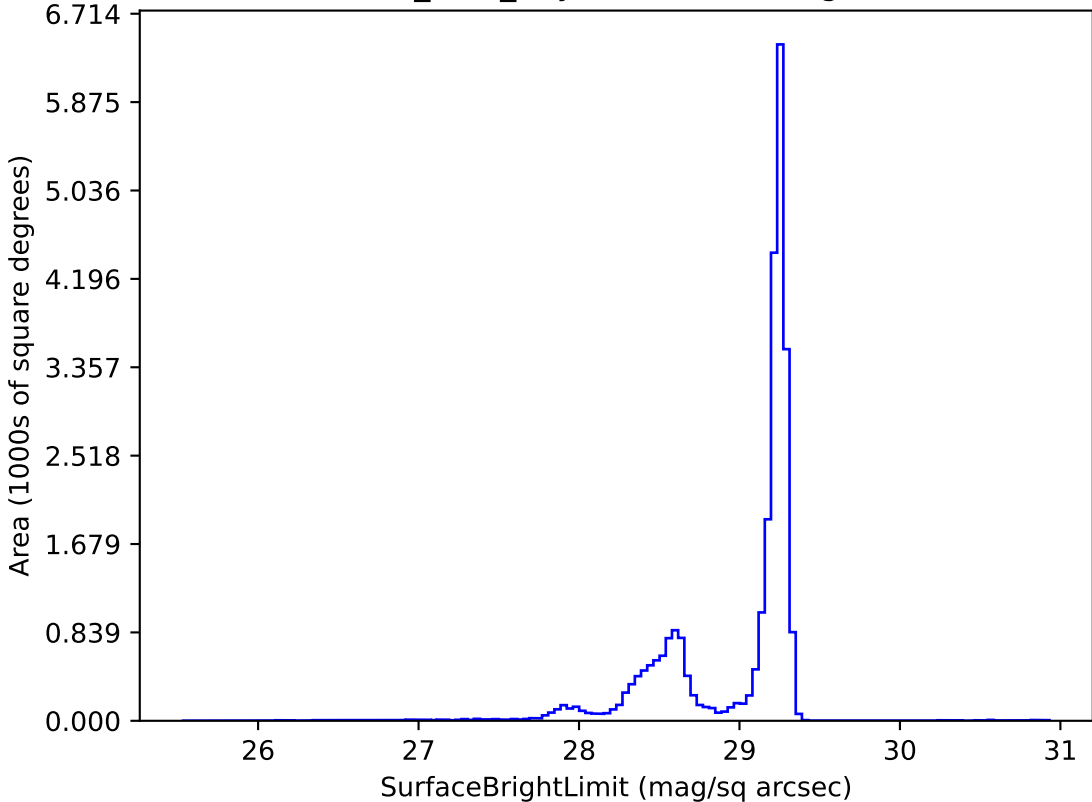
baseline_v2.2_10yrs z: SurfaceBrightLimit
