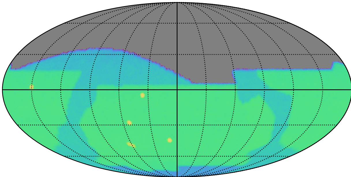
baseline_v2.2_10yrs z: SurfaceBrightLimit
