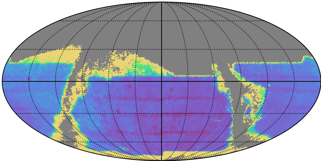
baseline_v2.2_10yrs : TDC_accuracy
