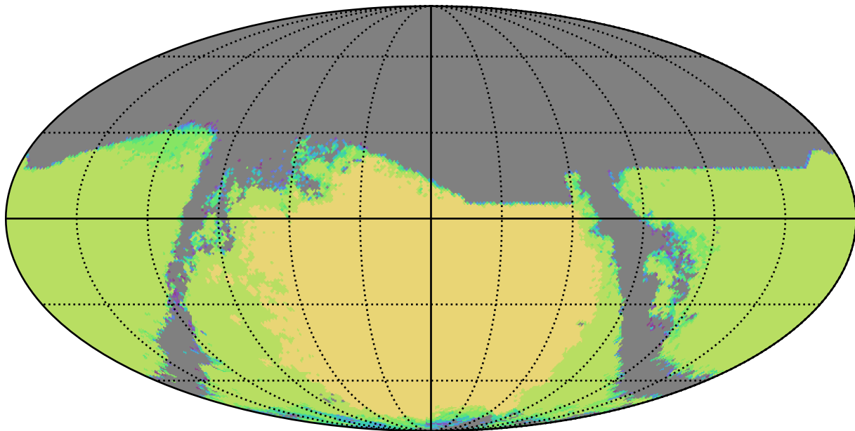
baseline_v2.2_10yrs : TDC_campaign
