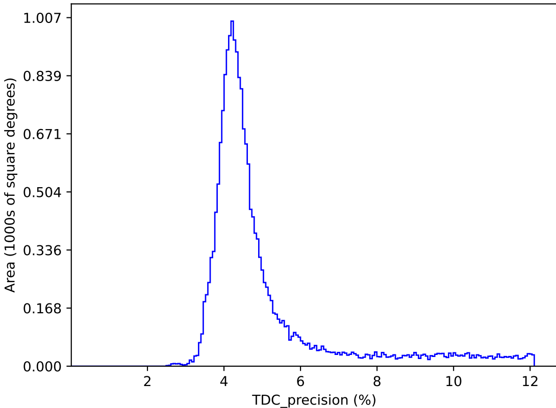
baseline_v2.2_10yrs : TDC_precision
