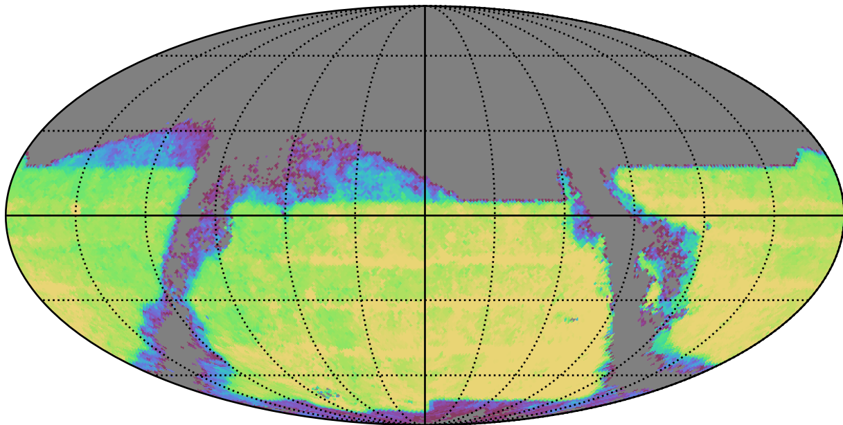
baseline_v2.2_10yrs : TDC_season
