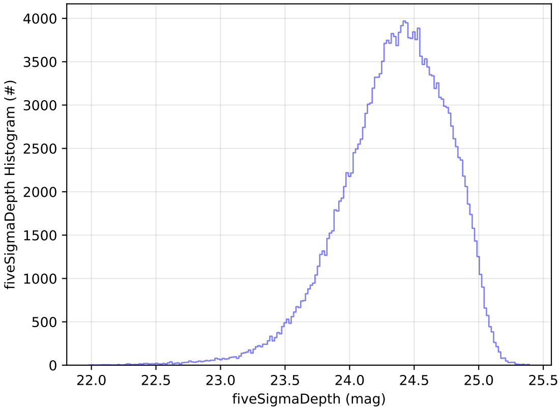
baseline_v2.2_10yrs g: fiveSigmaDepth Histogram
