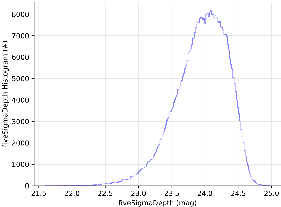
baseline_v2.2_10yrs r: fiveSigmaDepth Histogram
