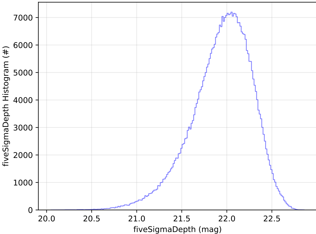
baseline_v2.2_10yrs y: fiveSigmaDepth Histogram
