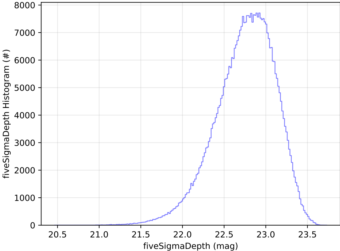
baseline_v2.2_10yrs z: fiveSigmaDepth Histogram
