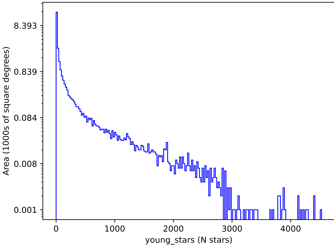
baseline_v2.2_10yrs : young_stars
