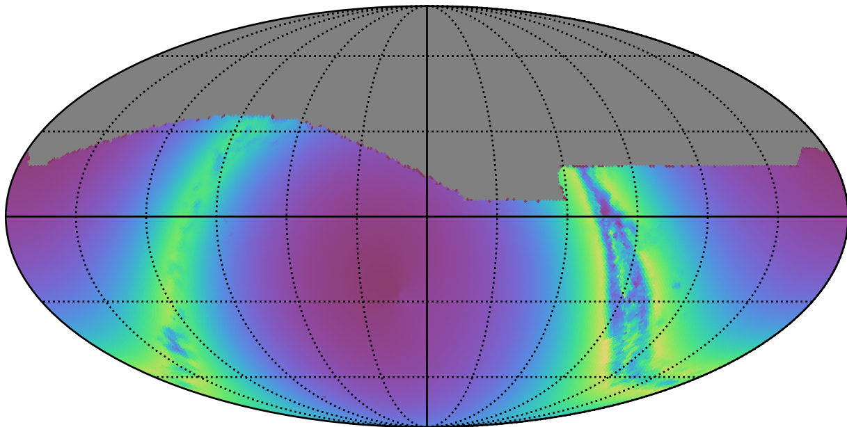
baseline_v2.2_10yrs : young_stars
