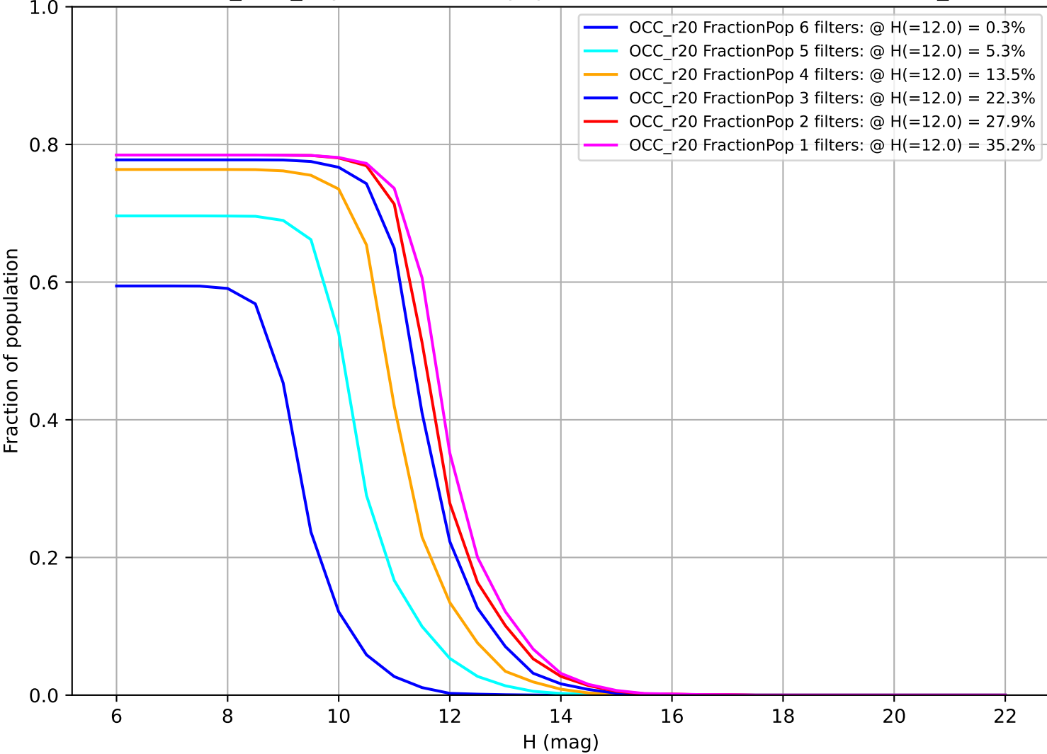
baseline_v2.2_10yrs: Fraction of population with colors in X filters OCC_r20
