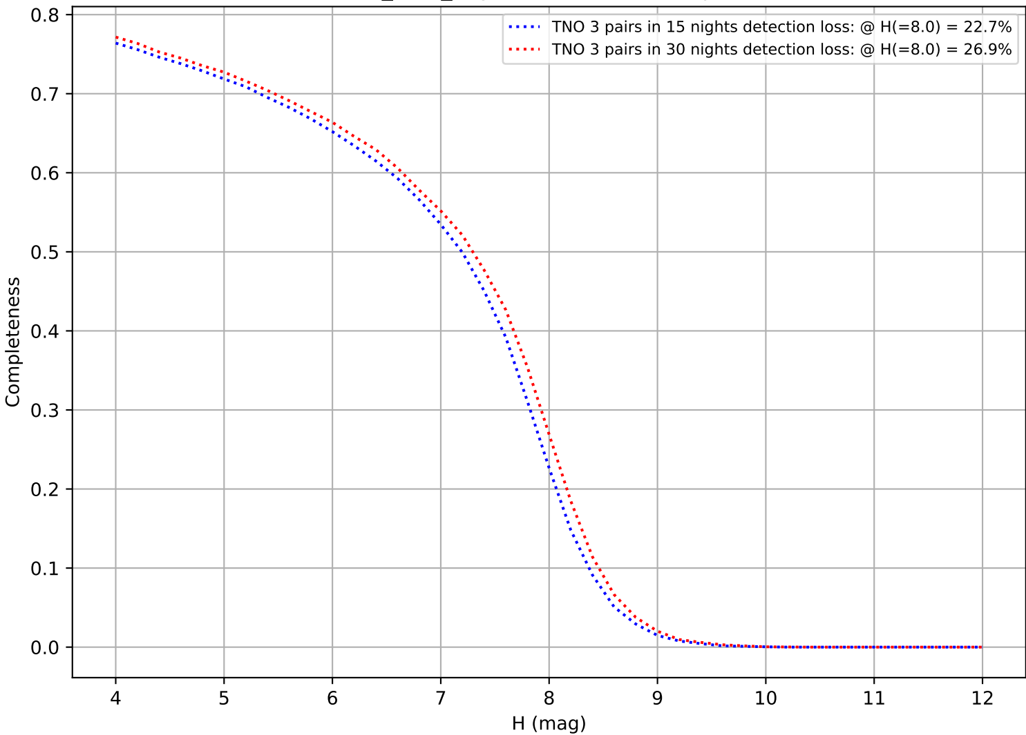
baseline_v2.2_10yrs: DifferentialCompleteness
