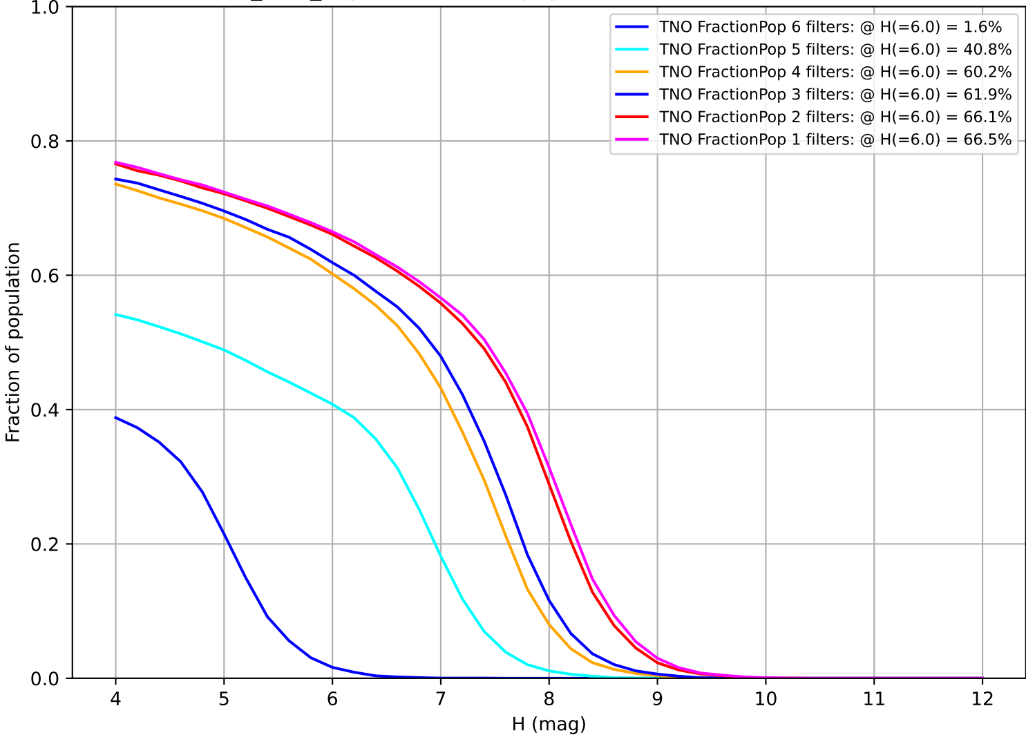
baseline_v2.2_10yrs: Fraction of population with colors in X filters TNO
