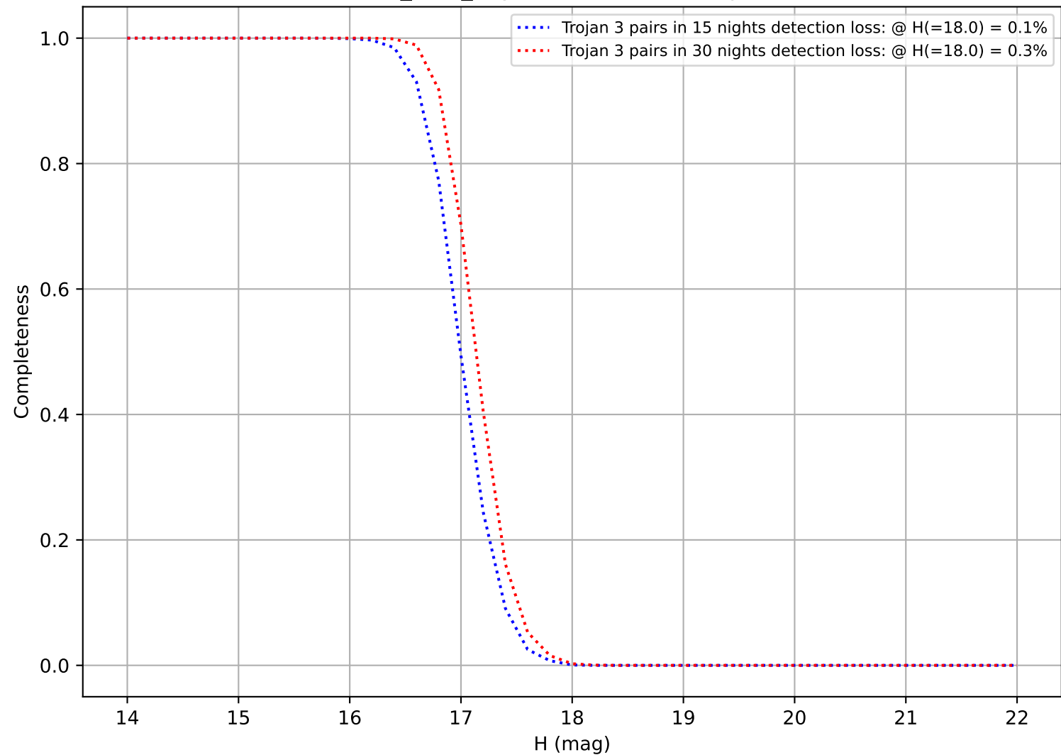
baseline_v2.2_10yrs: DifferentialCompleteness
