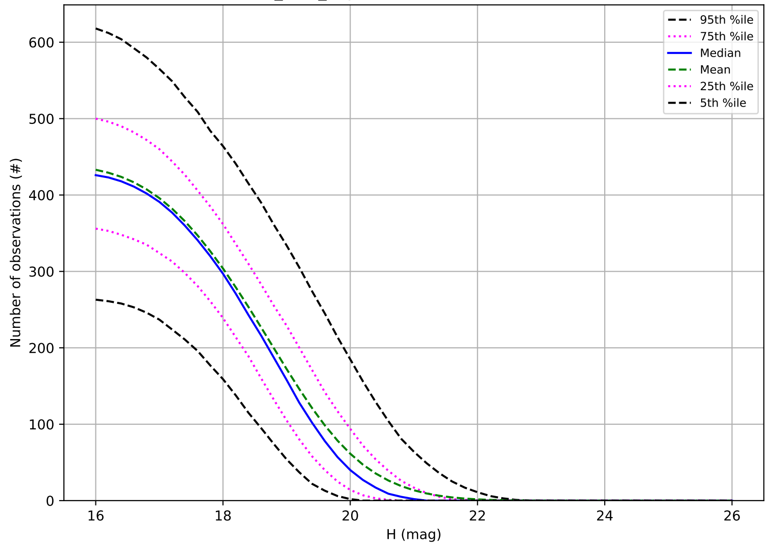
baseline_v2.2_10yrs: Number of observations MBA
