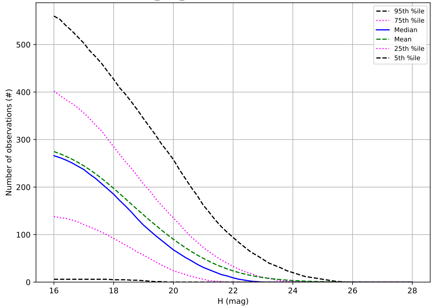
baseline_v2.2_10yrs: Number of observations NEO
