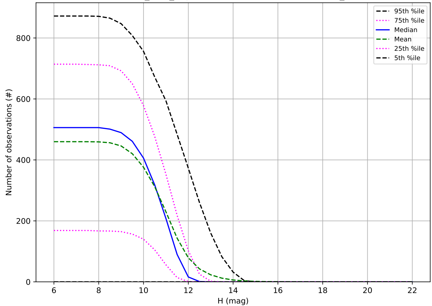
baseline_v2.2_10yrs: Number of observations OCC_r20
