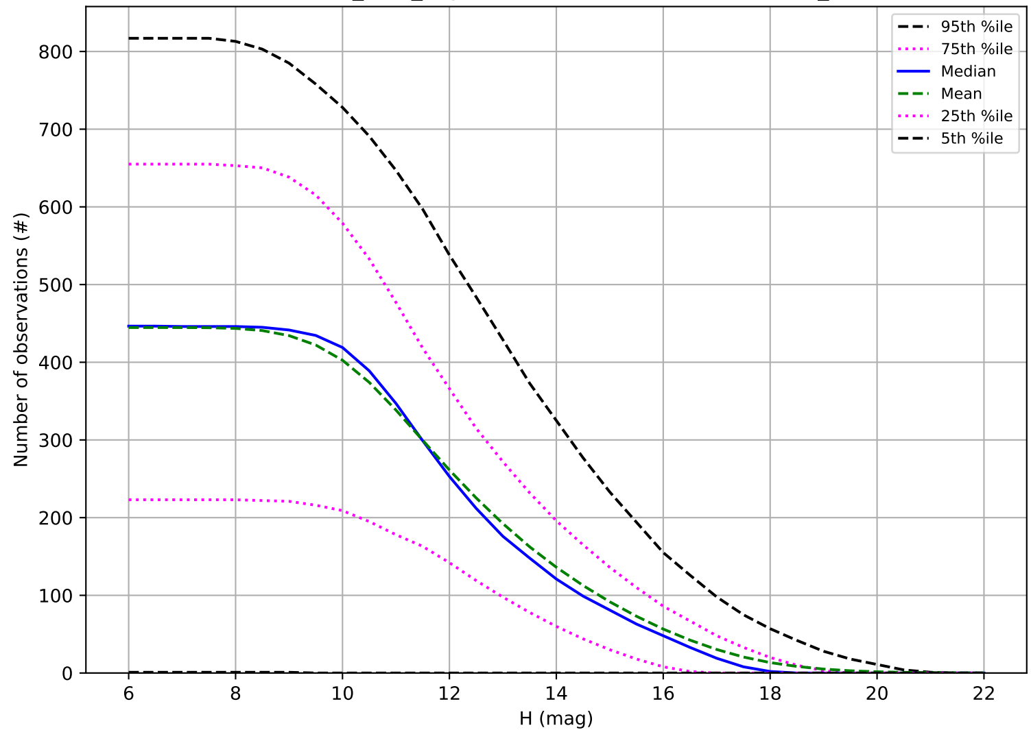
baseline_v2.2_10yrs: Number of observations OCC_r5
