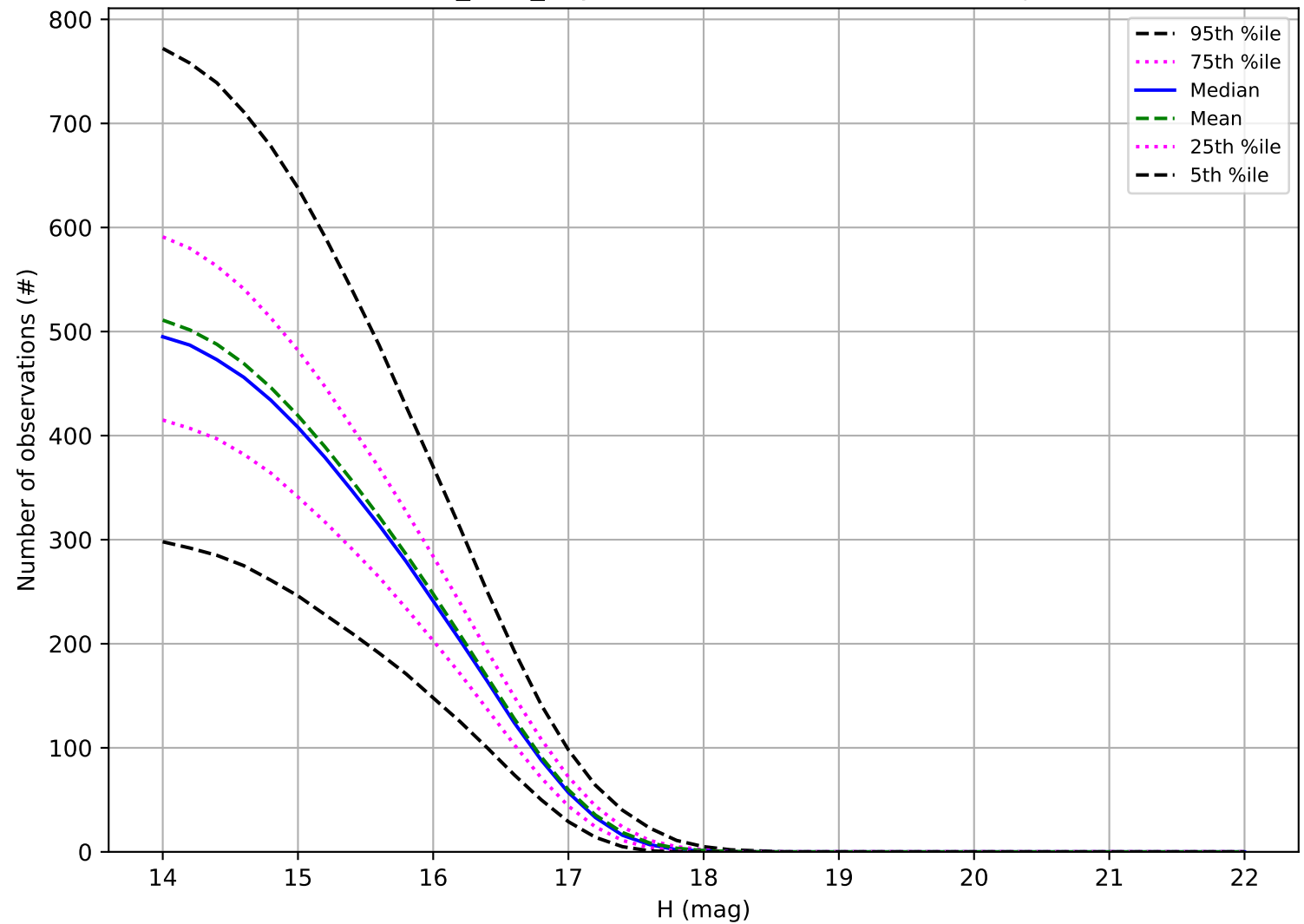
baseline_v2.2_10yrs: Number of observations Trojan
