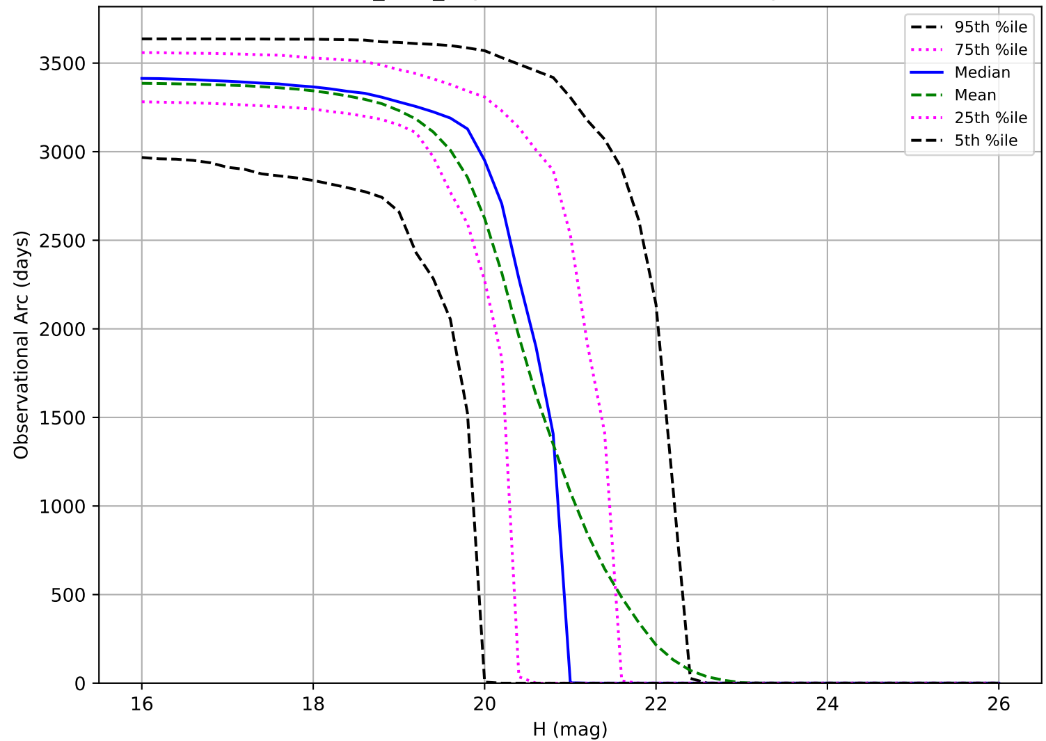
baseline_v2.2_10yrs: Observational Arc Length MBA
