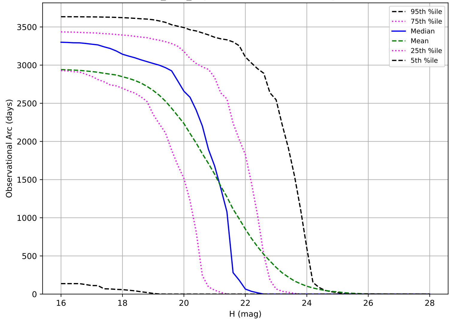
baseline_v2.2_10yrs: Observational Arc Length NEO
