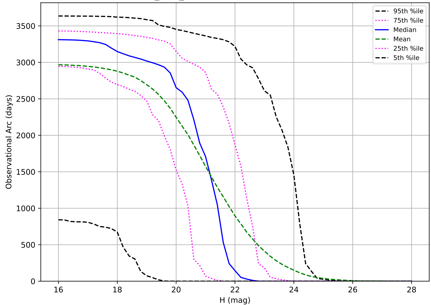
baseline_v2.2_10yrs: Observational Arc Length PHA
