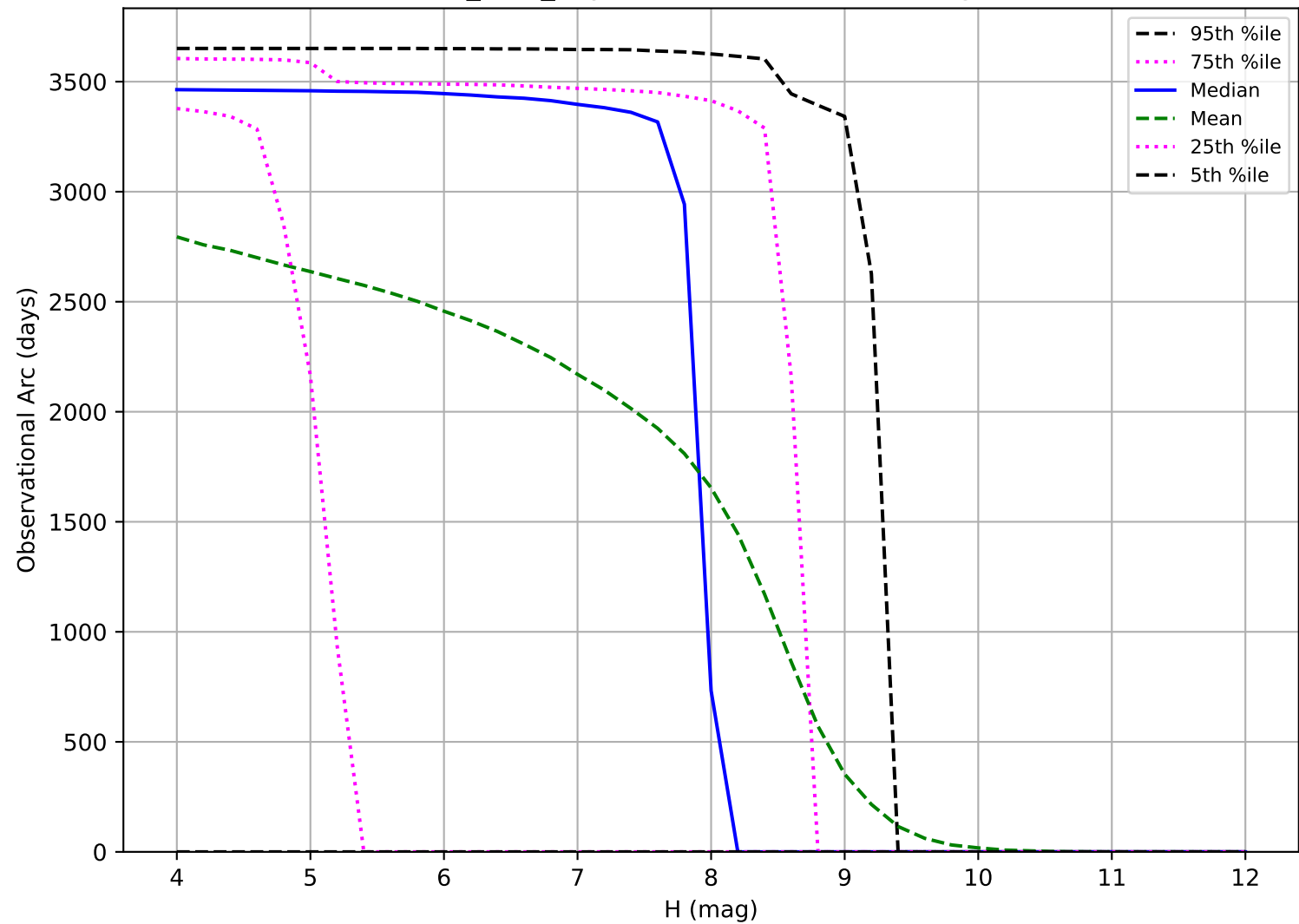
baseline_v2.2_10yrs: Observational Arc Length TNO
