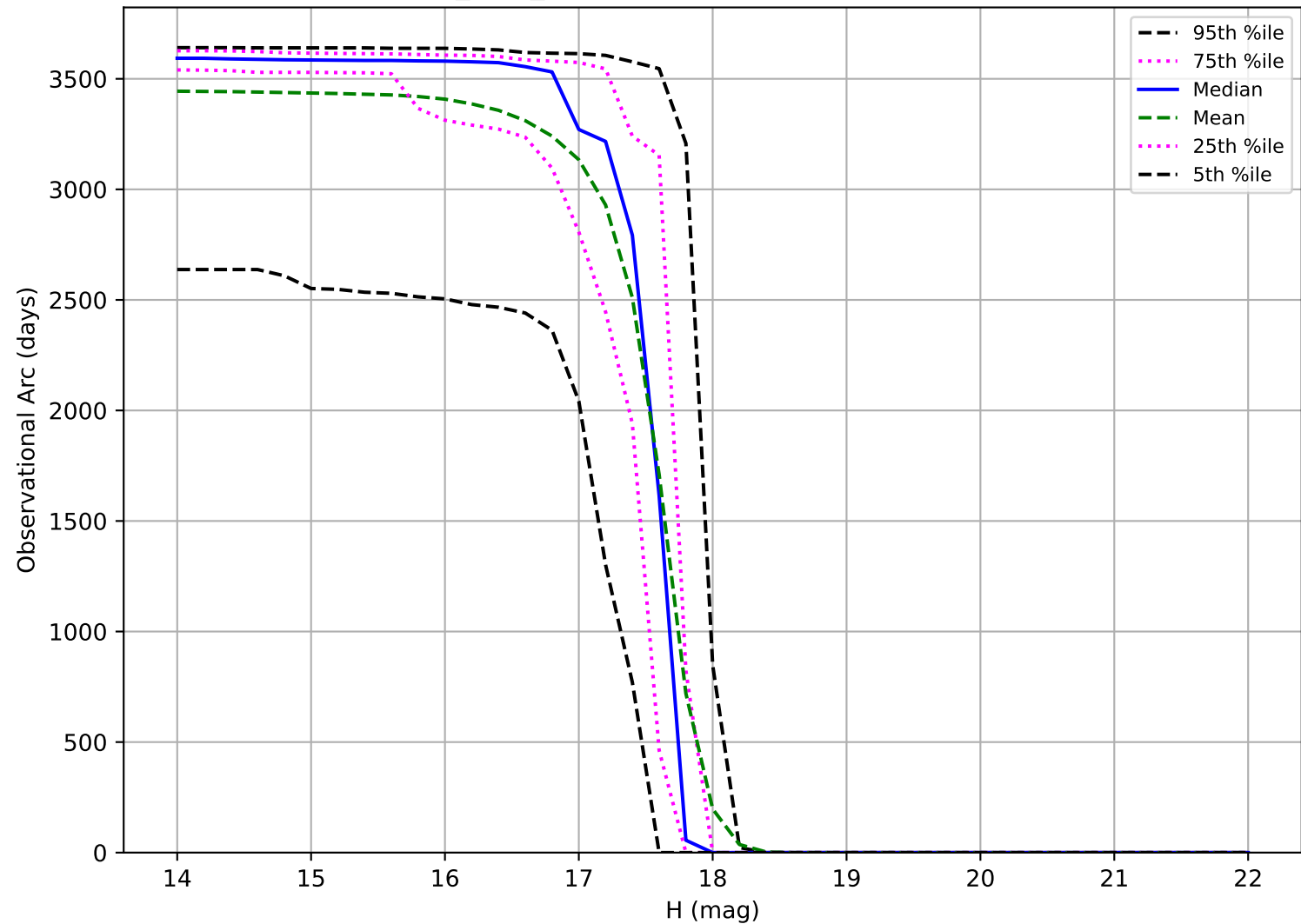
baseline_v2.2_10yrs: Observational Arc Length Trojan
